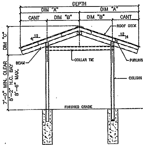
(A) CANOPY CROSS SECTION
