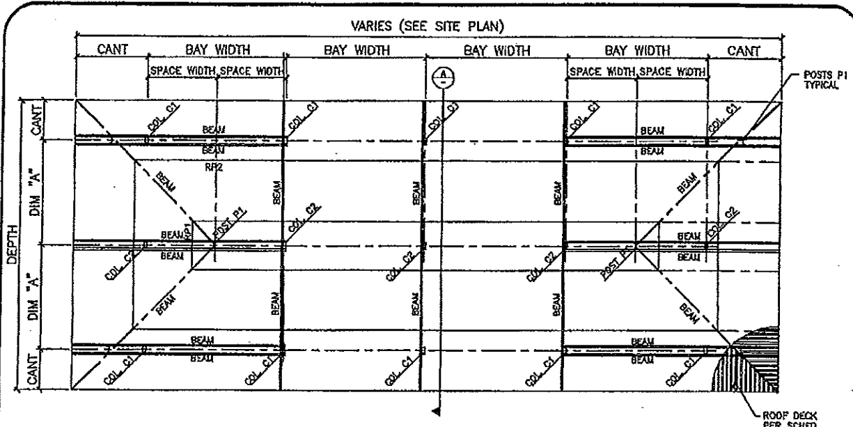
HR-BB ROOF FRAMING PLAN
