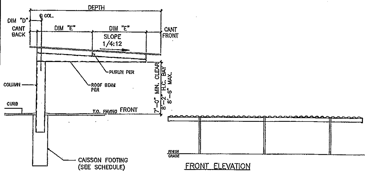
A FULL CANT CROSS SECTION
