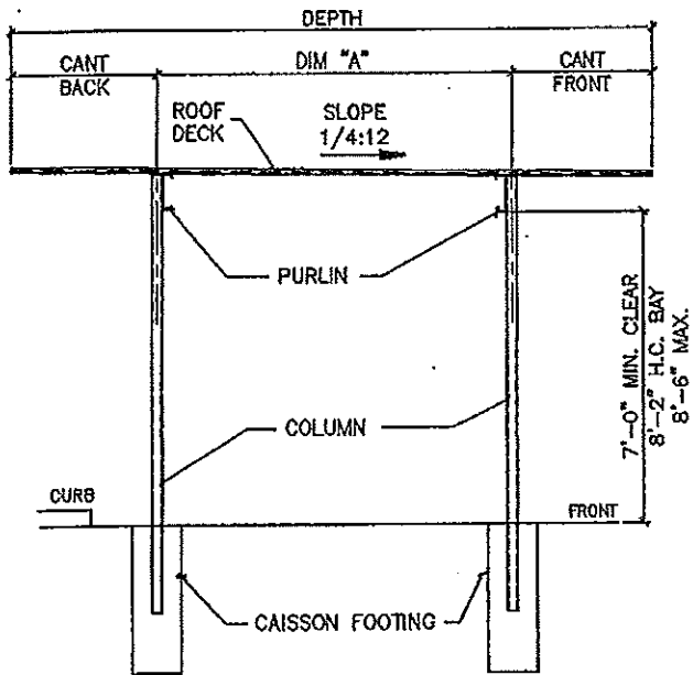
A DP CROSS SECTION
