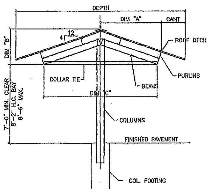
A SP GABLE CROSS SECTION
