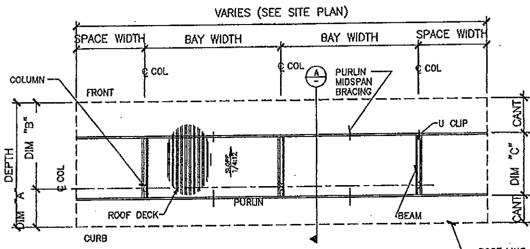
BSP 1/3 BACK ROOF FRAMING PLAN
