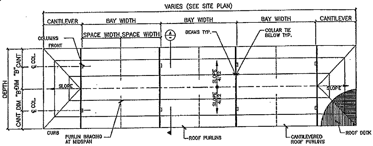
HR ROOF FRAMING PLAN
