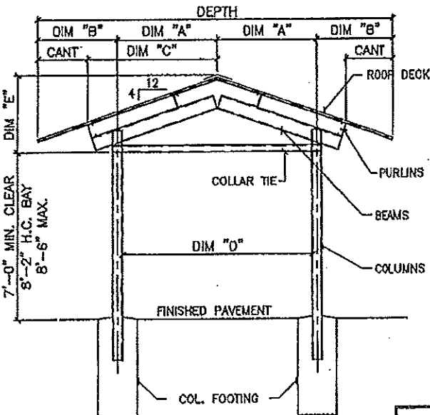
A GABLE CROSS SECTION
