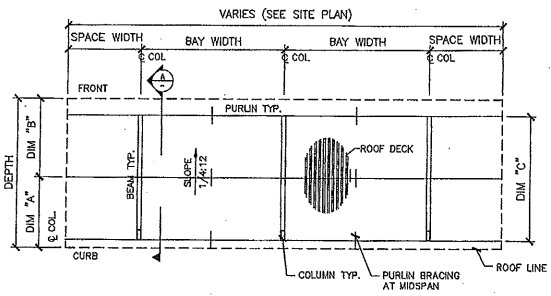
FULL CANT ROOF FRAMING PLAN
