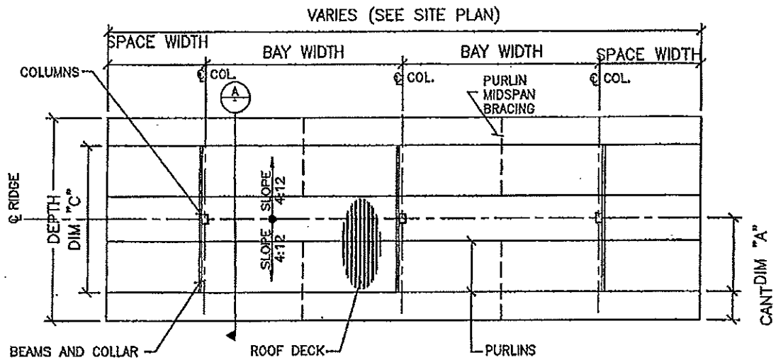
SP GABLE ROOF FRAMING PLAN
