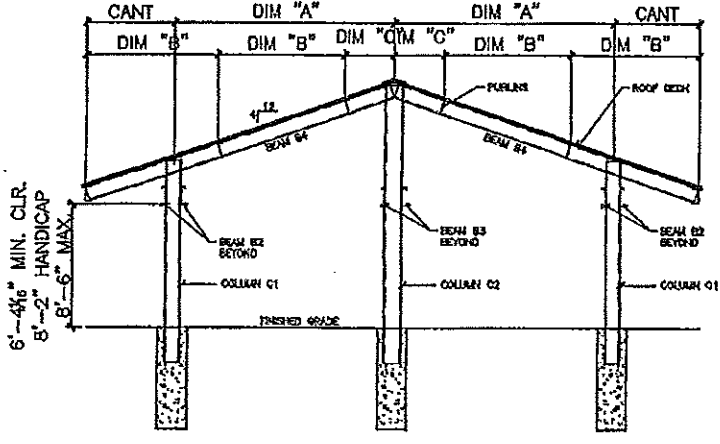
(A) HR-BB CROSS SECTION
