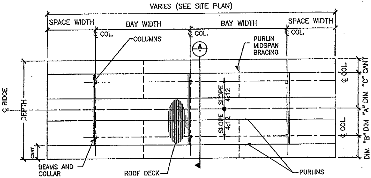
GABLE ROOF FRAMING PLAN
