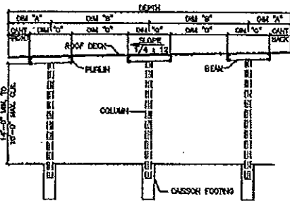
A CROSS SECTION 11x40
