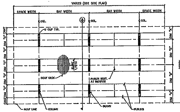
RV 90DEG ROOF FRAMING PLAN
