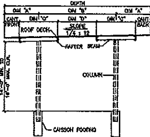
A CROSS SECTION 11x30
