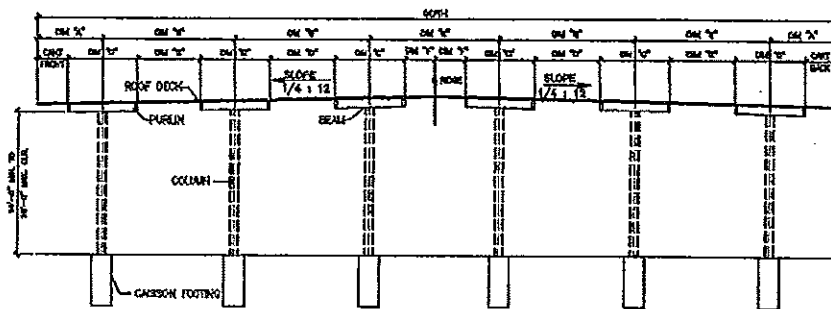
A CROSS SECTION 11x80
