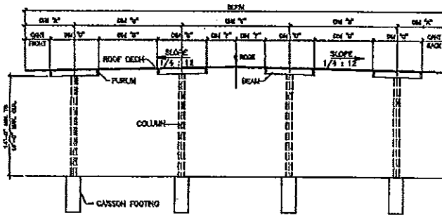
A CROSS SECTION 11x60
